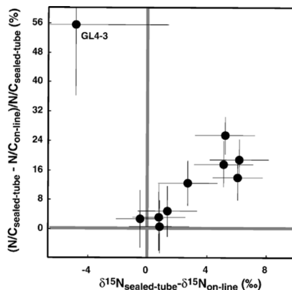
Fig. 2. Results acquired by on-line and sealed-tube combustion methods are compared by plotting \text{a}^{15}\text{N} \cdot \text{a}^{15}\text{N}_{\text{sealed-tube}} - \text{a}^{15}\text{N}_{\text{on-line}} versus \text{AN} / \text{C} = (\text{N} / \text{C}_{\text{sealed-tube}} - \text{N} / \text{C}_{\text{on-line}}) / \text{N} / \text{C}_{\text{sealed-tube}} . All the points should fall close to zero on both scales if both methods were giving the same results.
