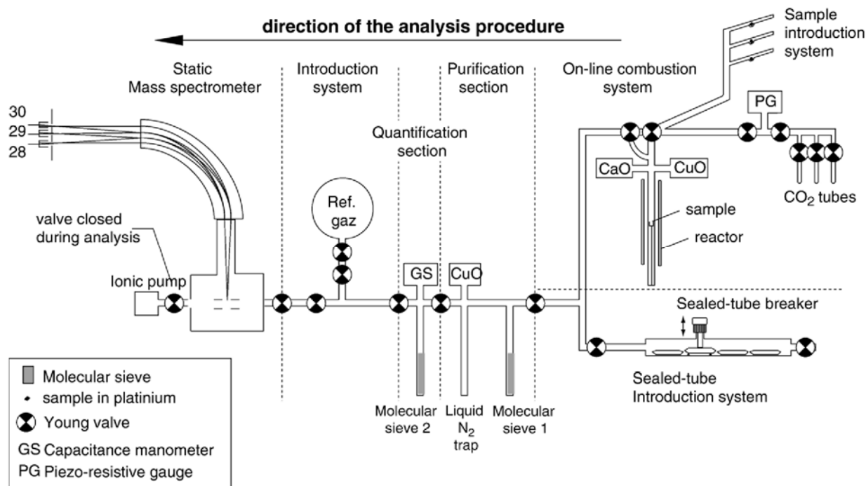
Fig. 1. Schematic representation of the ultra high-vacuum line.
