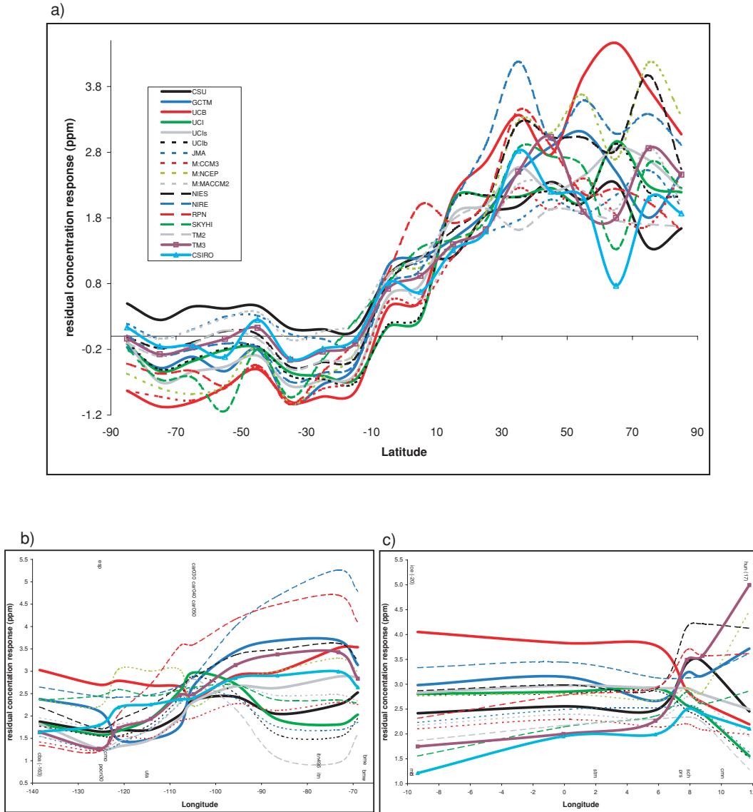
Fig. 4. (a) Smoothed (mean of 10° latitudinal bins) residual concentration response (ppm) at the 76 CO 2 observational stations for each of the models. (b) Smoothed (three station running mean) residual concentration response (ppm) at North American stations within the 30°N to 70°N longitudinal band. Longitudes are listed for stations located outside the center of the running mean. (c) Same as (b) but for Europe.
