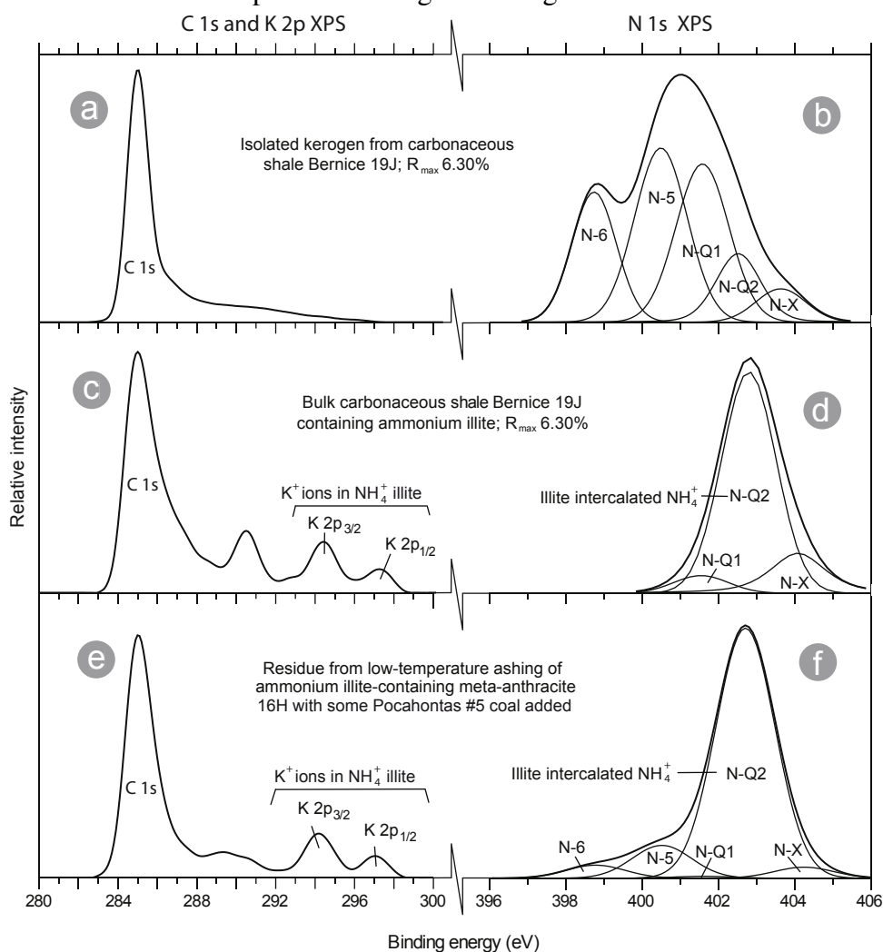
Fig. 5: N 1s XPS and C 1s XPS spectra with curve-fitted sub-peaks for: (a, b) kerogen isolated from carbonaceous shale Bernice 19J, a carbon-poor shale that was sampled close to an anthracite bed; (c, d) the same bulk carbonaceous shale Bernice 19J containing ammonium illite; and (e, f) the inorganic residue 16H-LTA from low-temperature plasma ashing of meta-anthracite 16H; the ash was mixed with a
