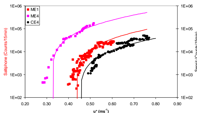
Fig. 5. Intensity of the saltation (in counts cumulated over 15 min) detected by the Saltiphone during ME1 and ME4, and by the Sensit during CE4.. Note that because they were not cross-calibrated the counts given by the two instruments cannot be compared numerically. The best fit of White's (1986) equation to the measurements is reproduced in each case.
