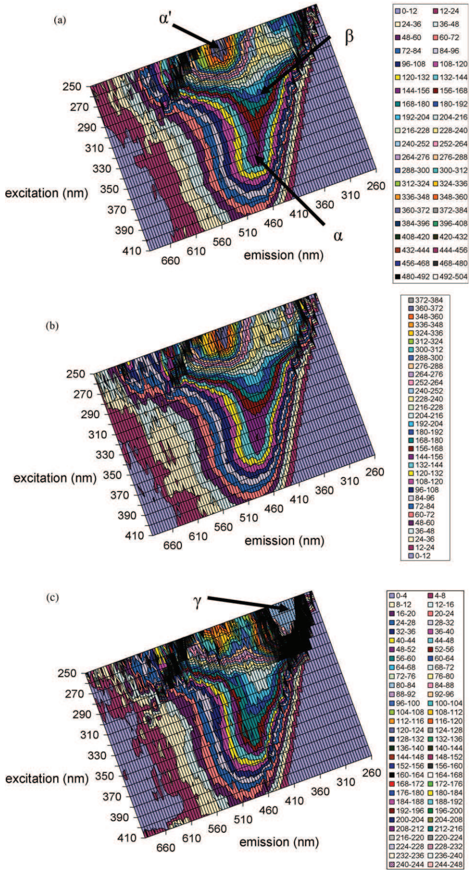
Fig. 4. Contour excitation–emission matrix plots of the initial Mediterranean seawater sample (a), of the diluate with a salinity of 22.9 (b) and of the diluate at the end of the electrodesalting (c) (desalting of 2 L of Mediterranean seawater). Fluorescence intensity scales identical for (a) and (b). Intensity scale three times smaller for (c) than for (a) and (b).
